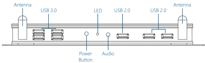
Front Panel
