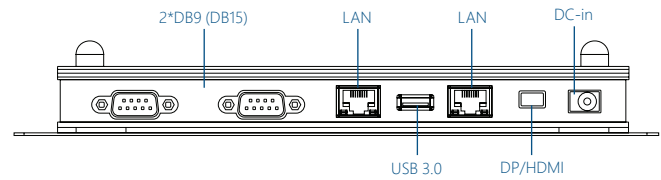
Rear Panel
