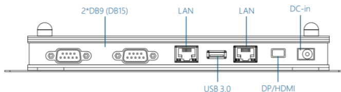
Rear Panel
